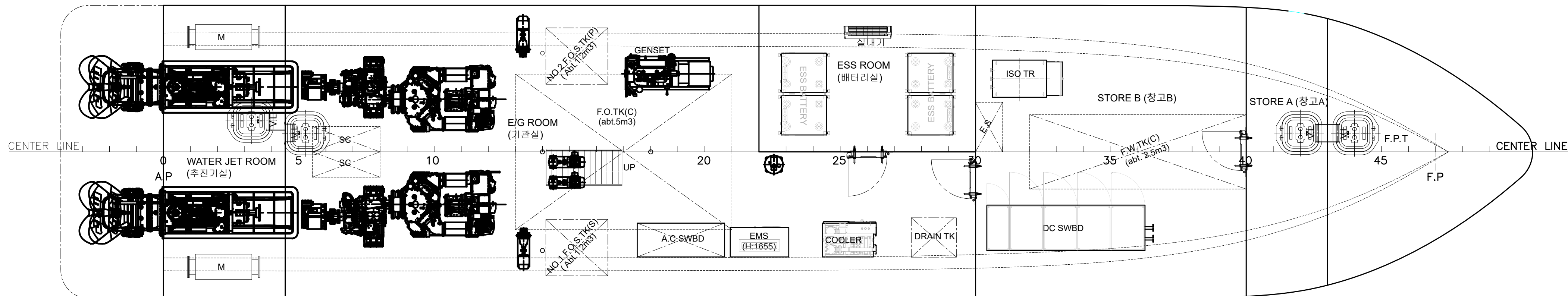
BOTTOM PLAN
